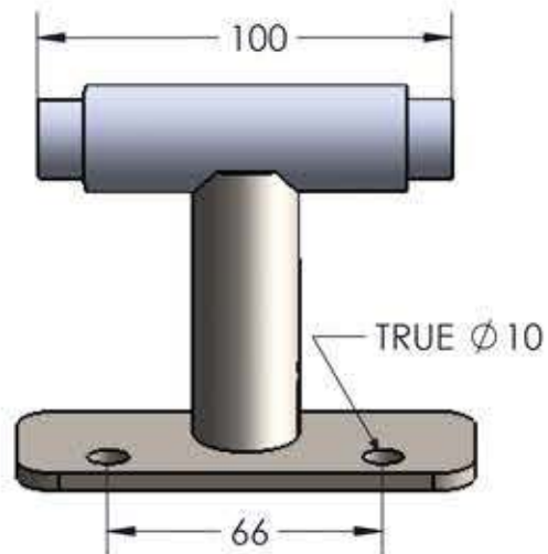
DRT15 AXLE SIZE 15MM X 100MM
